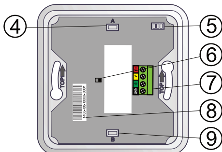
Figure 2: 4 – A button, 5 – LED indicator, 6 – Tamper contact, 7 – BUS terminals, 8 – Production code, 9 – B button
